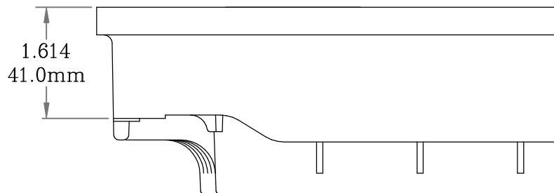
PARTIAL TOP VIEW (174.4 Sq. In. Open Area)
