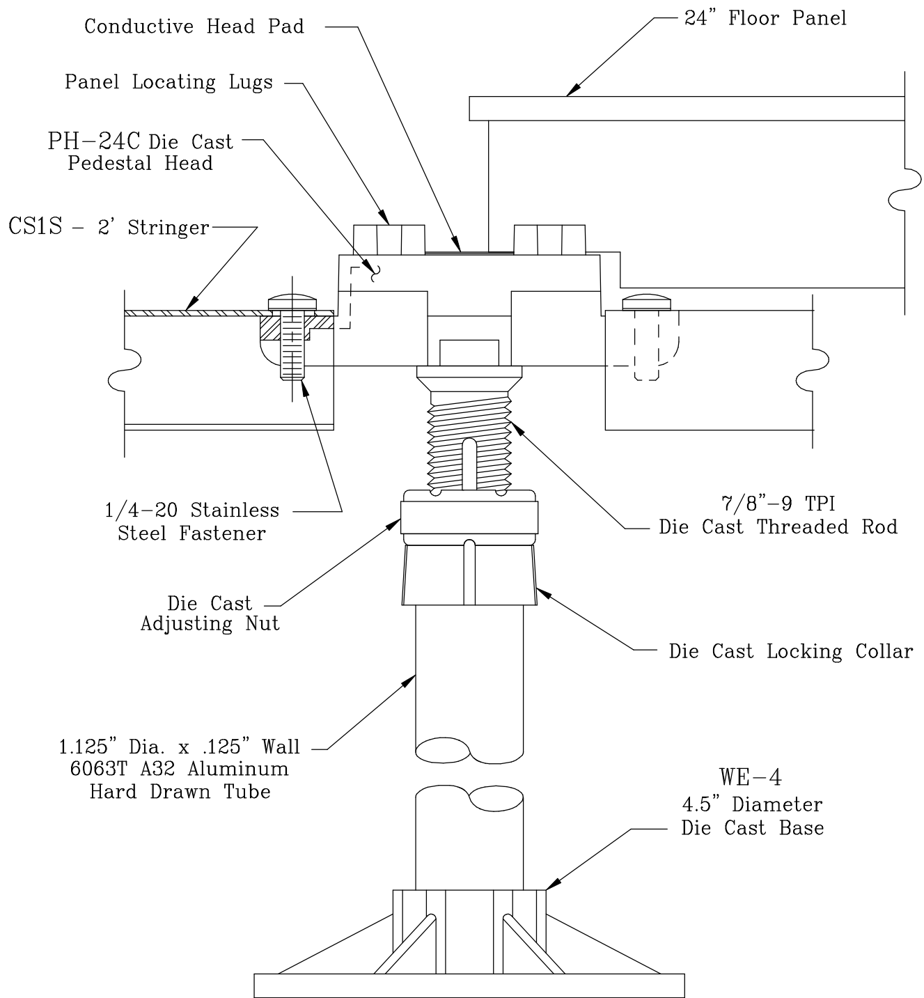
SIDE ELEVATION DETAIL
