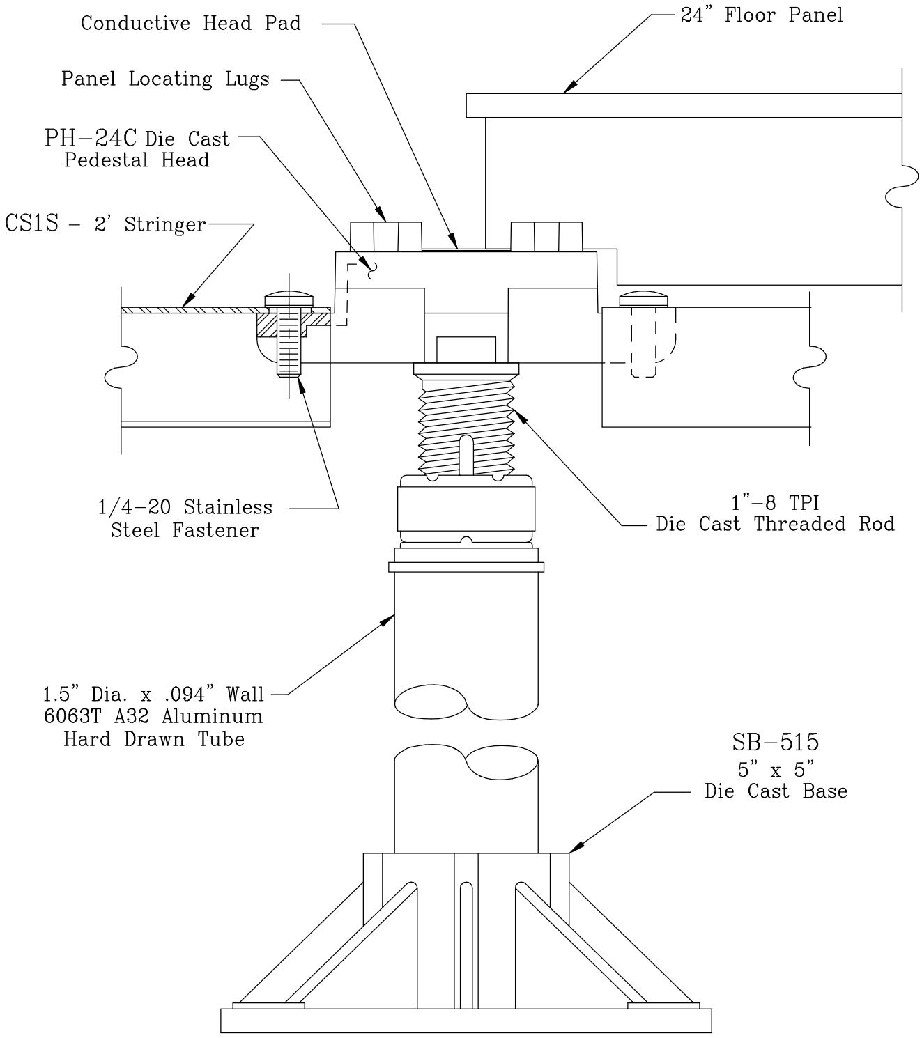
SIDE ELEVATION DETAIL
