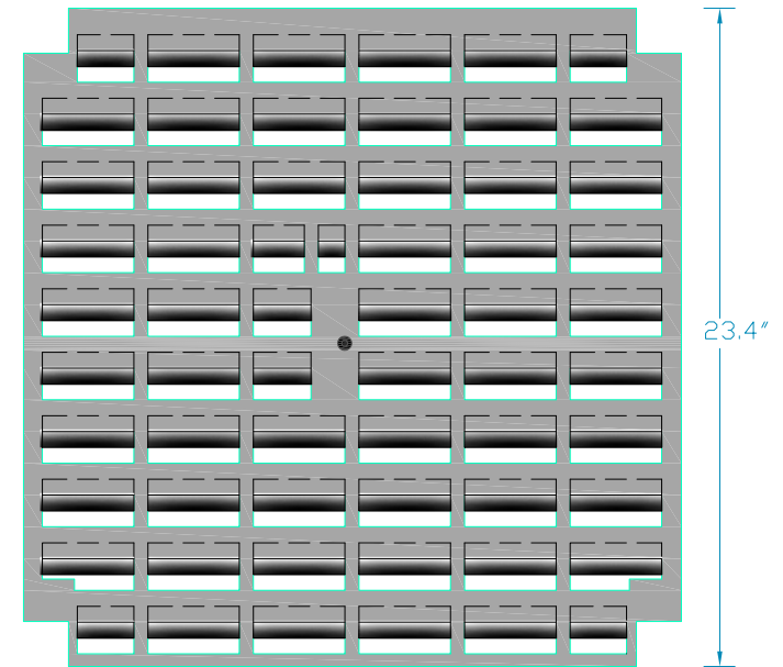
Top View of HR 24 Adjustable Damper
