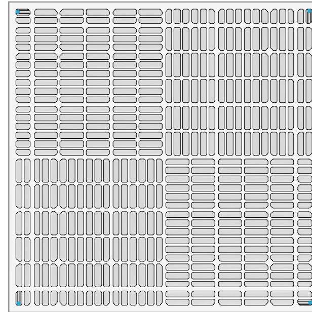
Top View of GP 24 Conductive Epoxy Coated Cornerlock Panel
